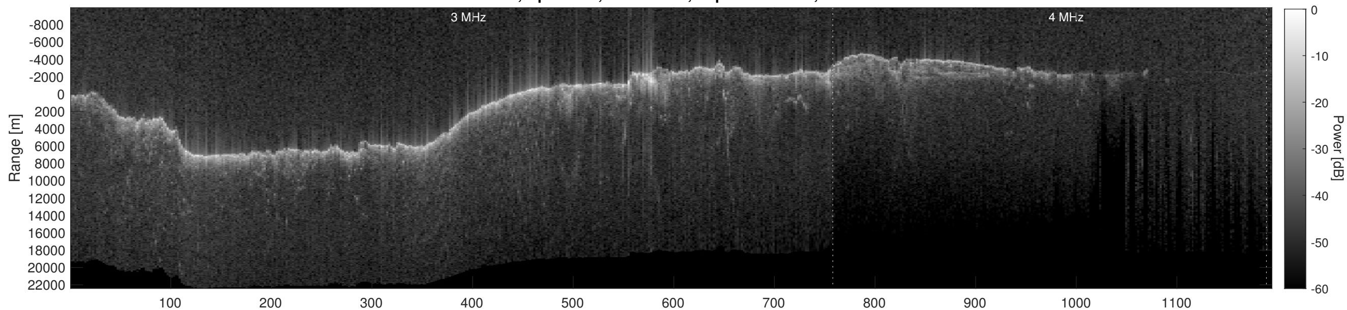
Orbit 8850, Depth-Corrected Cluttergram
