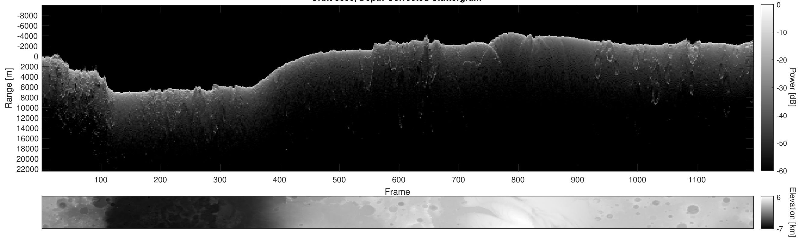
Orbit 8850, Depth-Corrected Cluttergram
