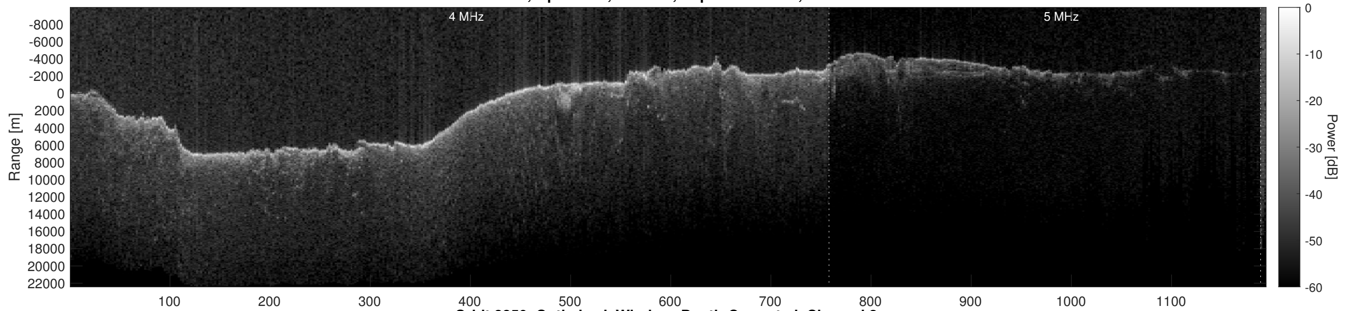
Orbit 8850, Optimized, Window, Depth-Corrected, Channel 2
