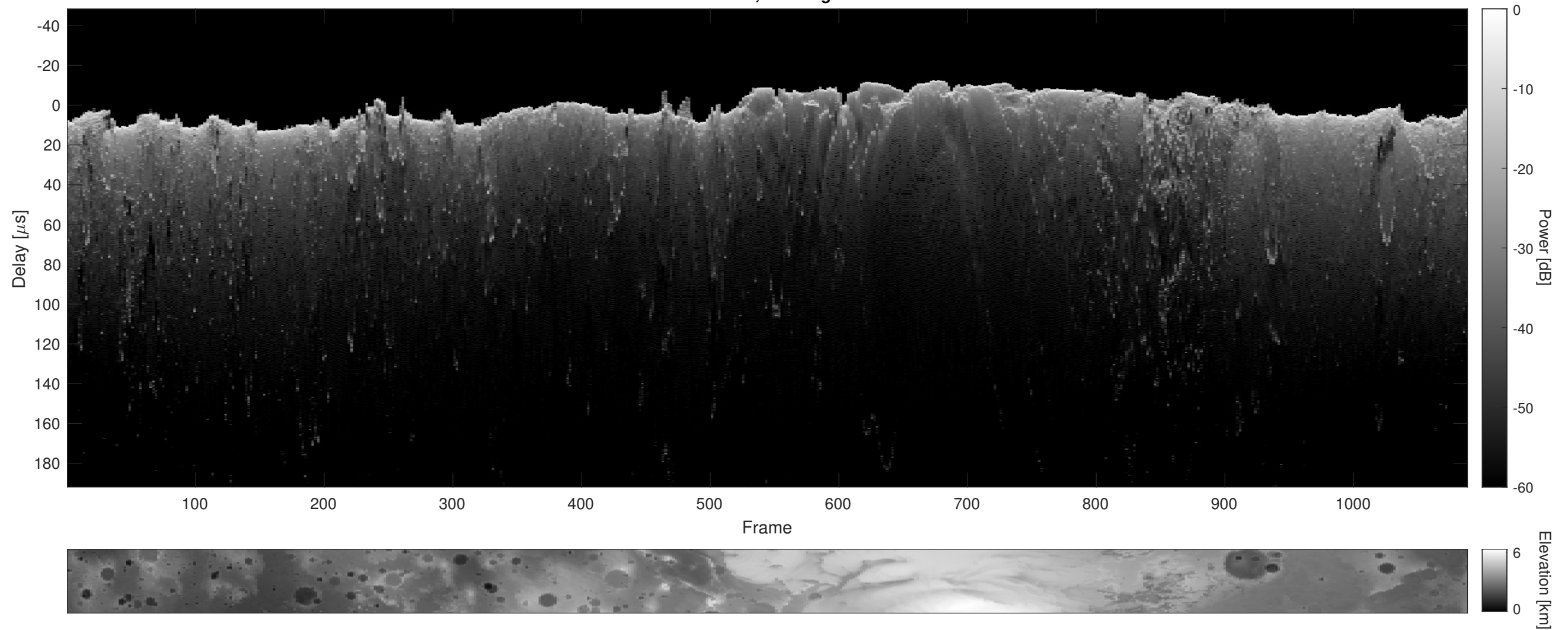
Orbit 8853, Cluttergram
