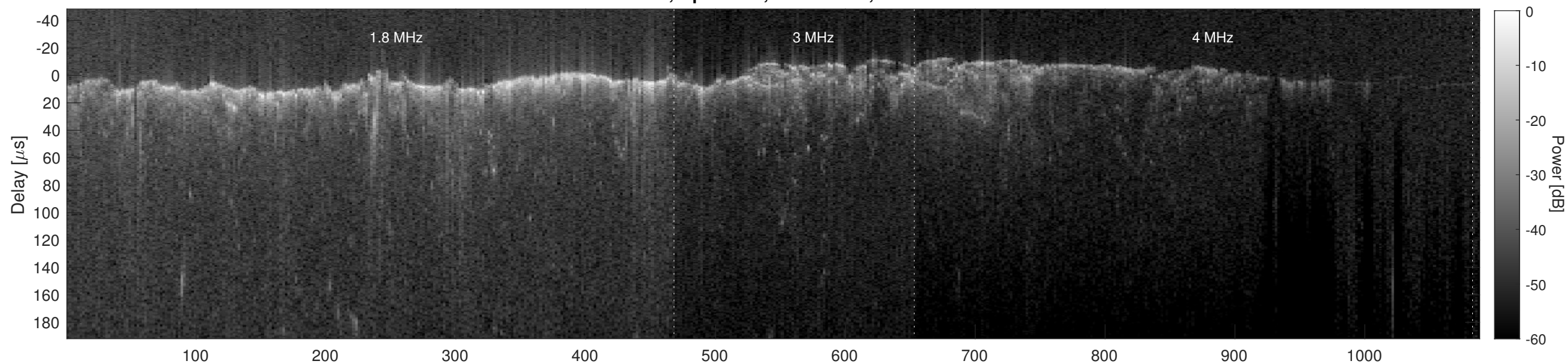
Orbit 8853, Cluttergram
