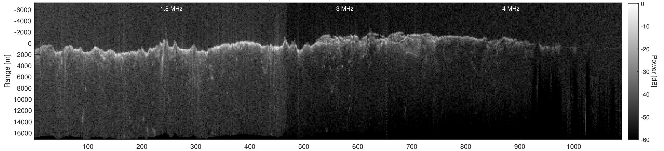
Orbit 8853, Depth-Corrected Cluttergram
