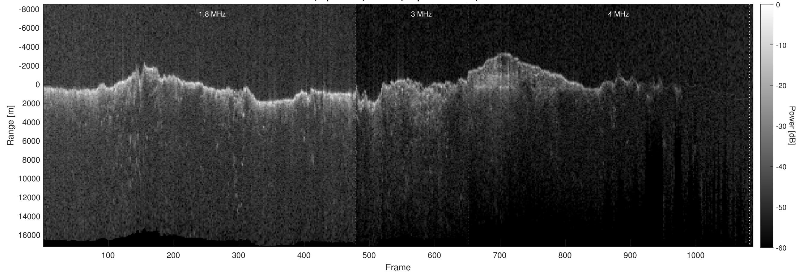
Orbit 8855, Optimized, Window, Depth-Corrected, Channel 2
