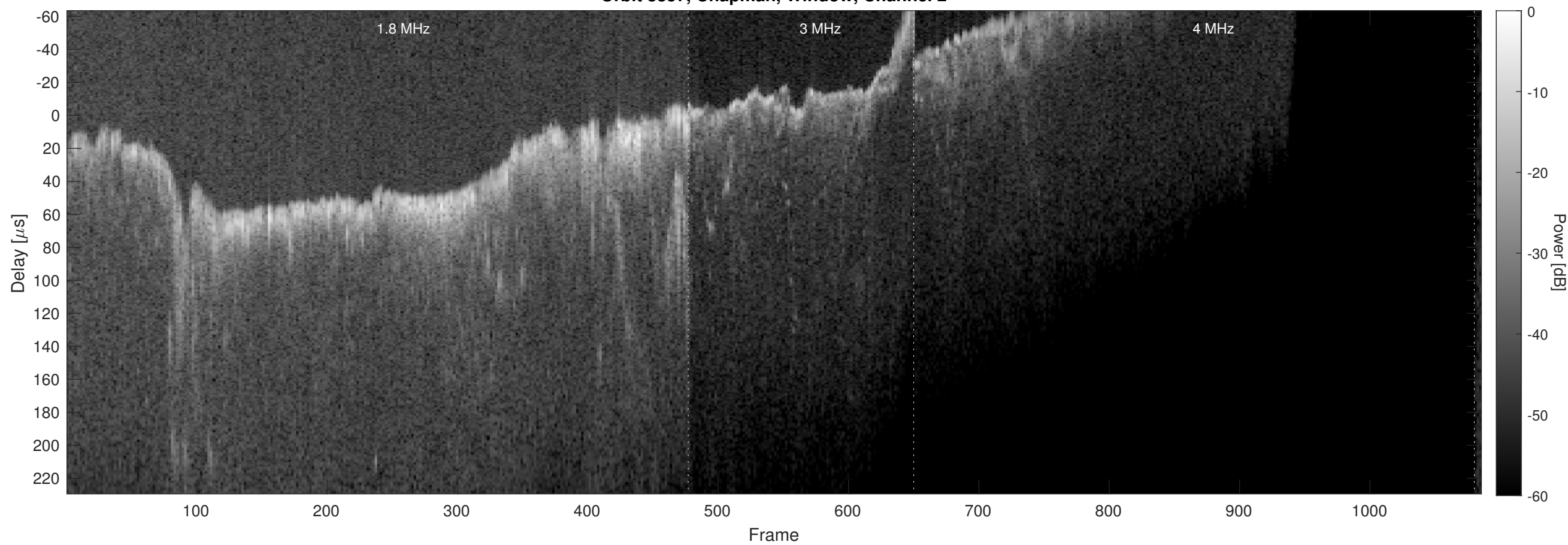
Orbit 8857, Chapman, Window, Channel 2
