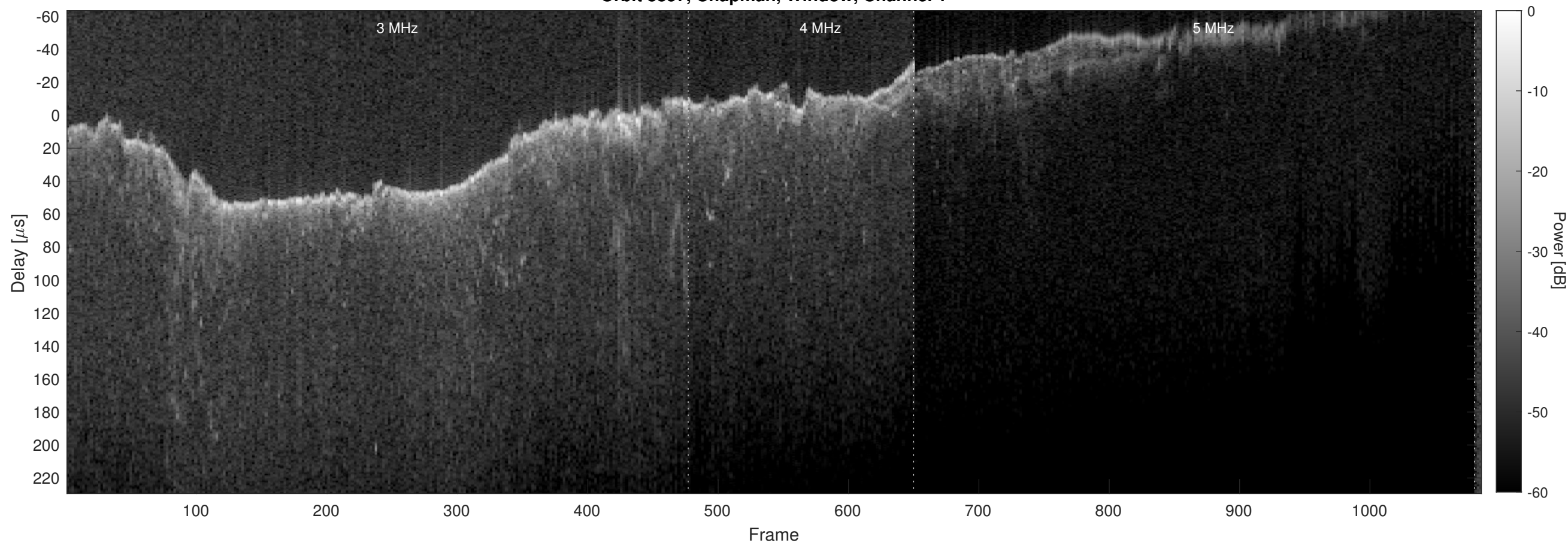
Orbit 8857, Chapman, Window, Channel 2
