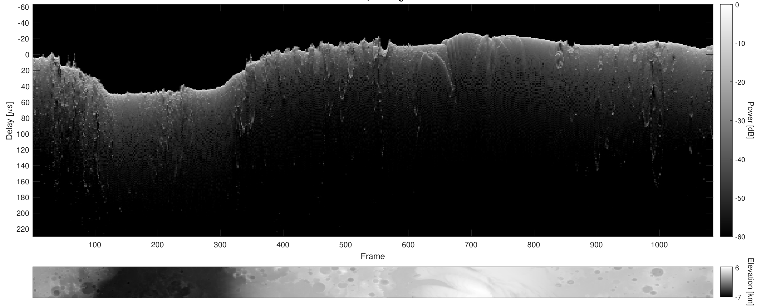
Orbit 8857, Cluttergram
