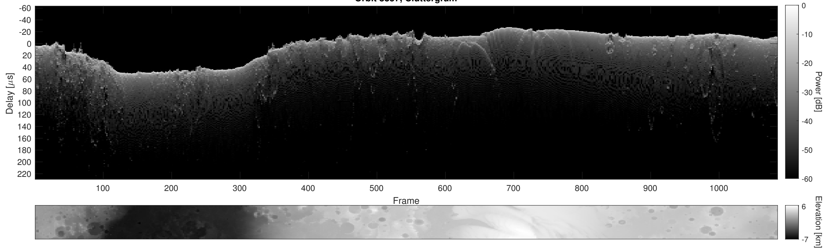
Orbit 8857, Cluttergram
