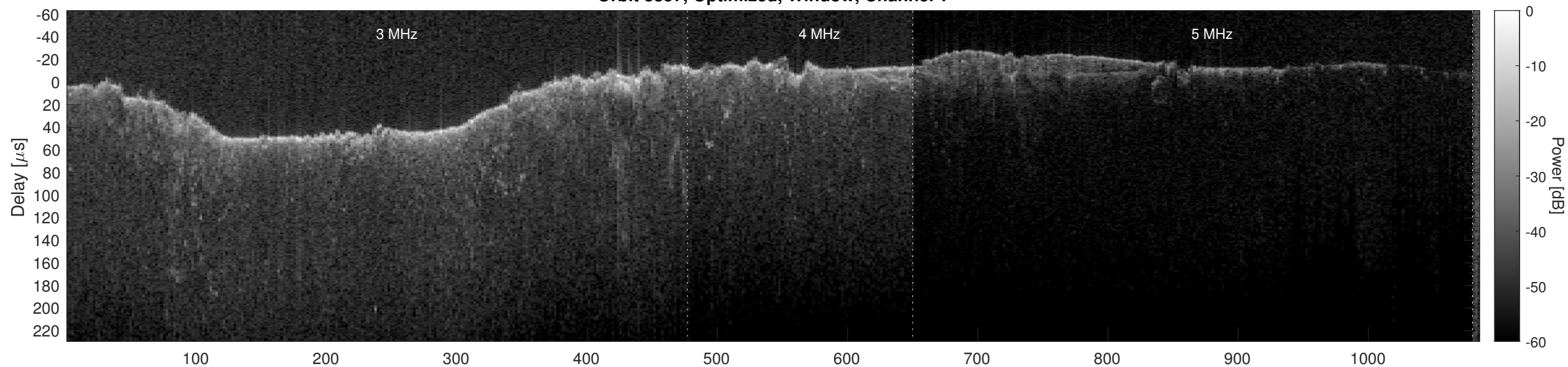
Orbit 8857, Optimized, Window, Channel 2
