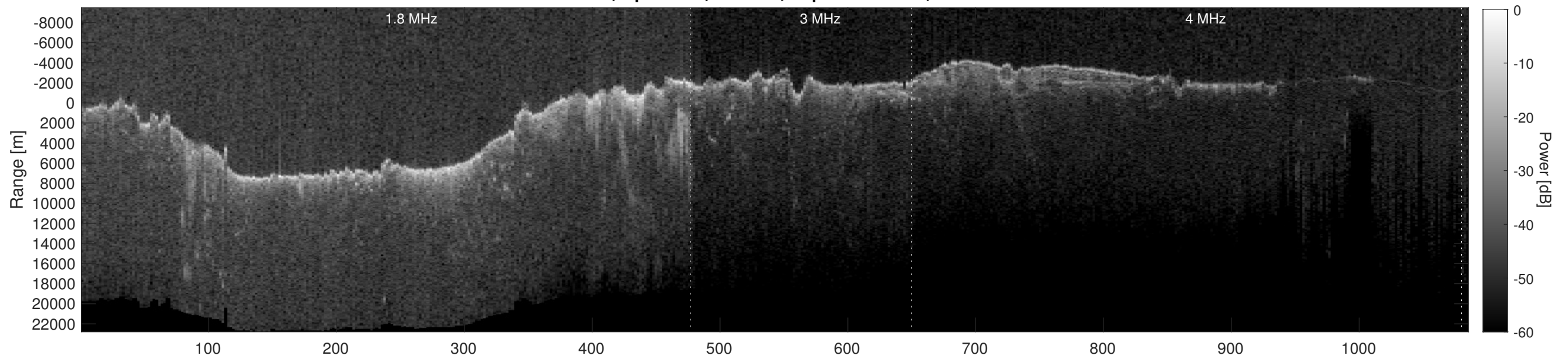
Orbit 8857, Depth-Corrected Cluttergram
