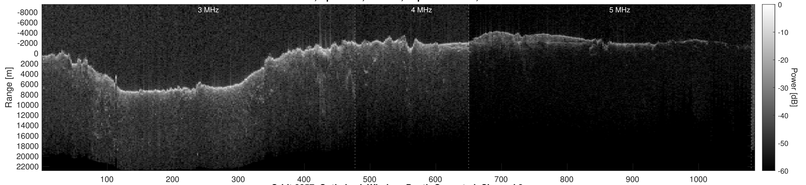
Orbit 8857, Optimized, Window, Depth-Corrected, Channel 2
