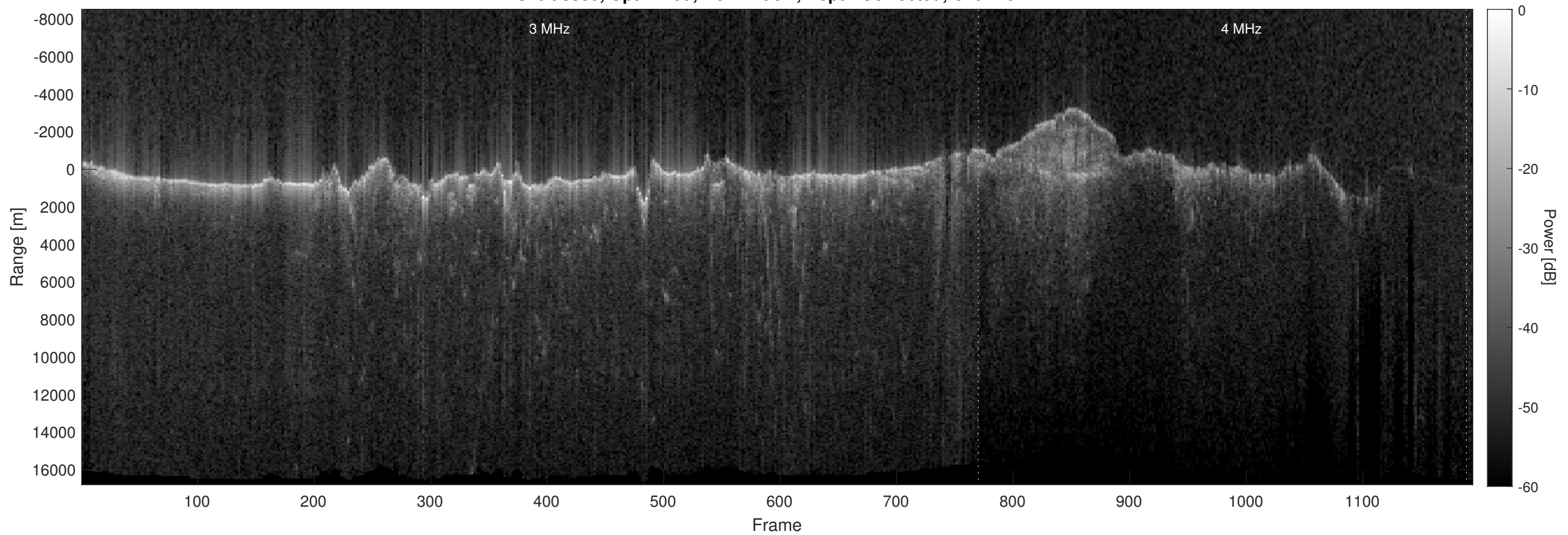
Orbit 8859, Optimized, No Window, Depth-Corrected, Channel 2
