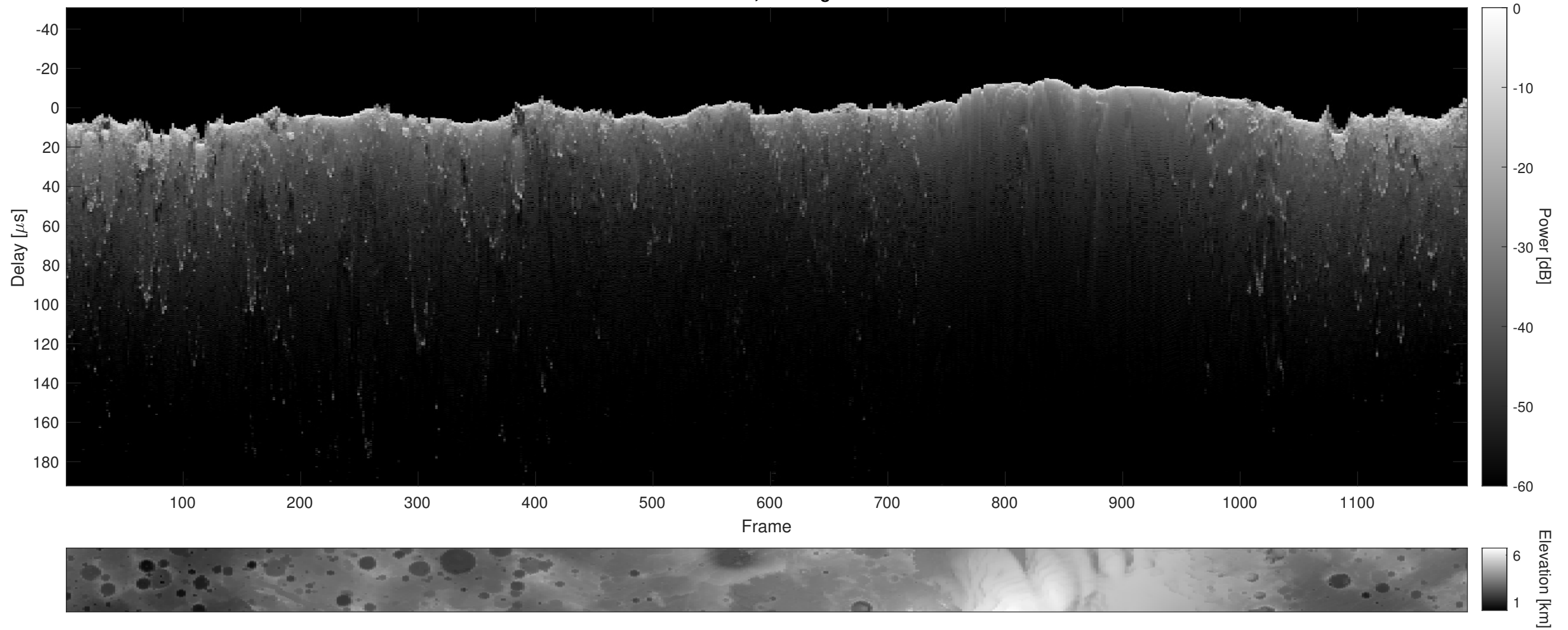
Orbit 8861, Cluttergram
