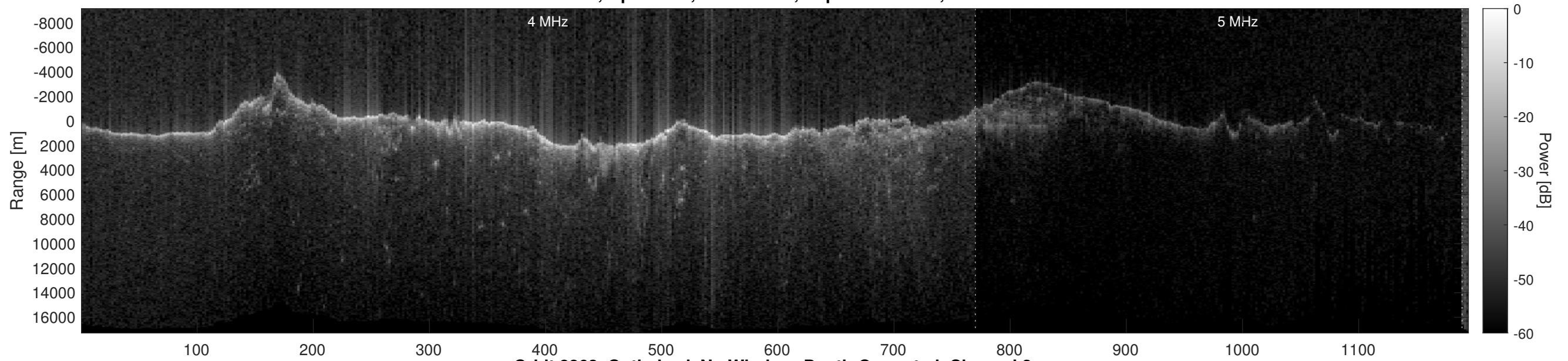
Orbit 8862, Optimized, No Window, Depth-Corrected, Channel 2
