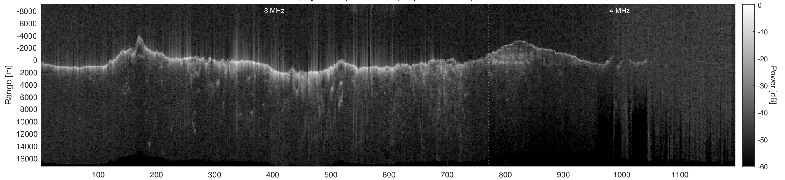
Orbit 8862, Depth-Corrected Cluttergram
