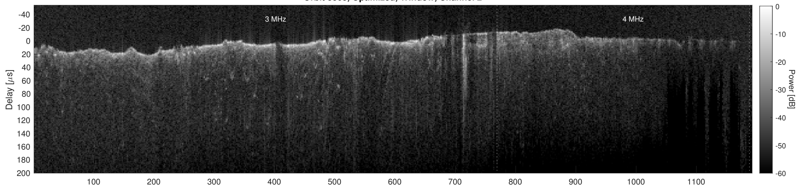
Orbit 8863, Cluttergram
