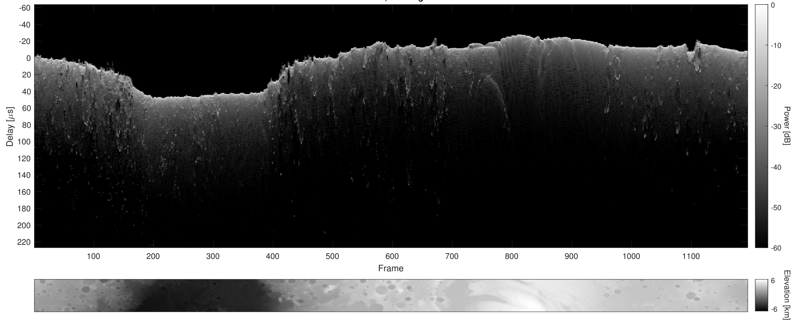
Orbit 8864, Cluttergram
