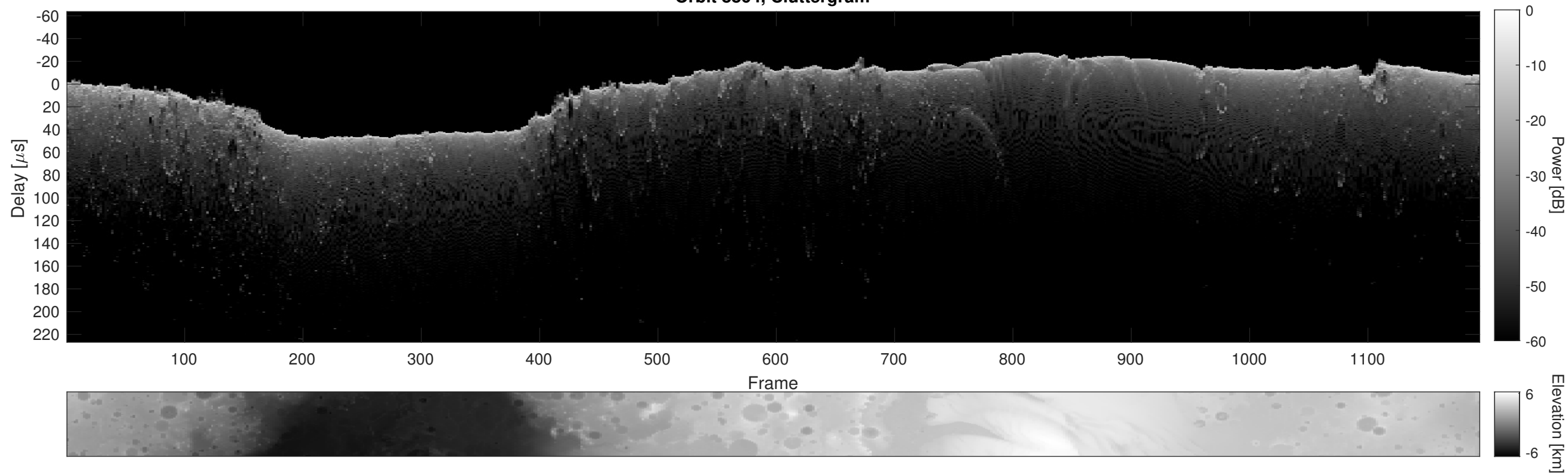
Orbit 8864, Cluttergram
