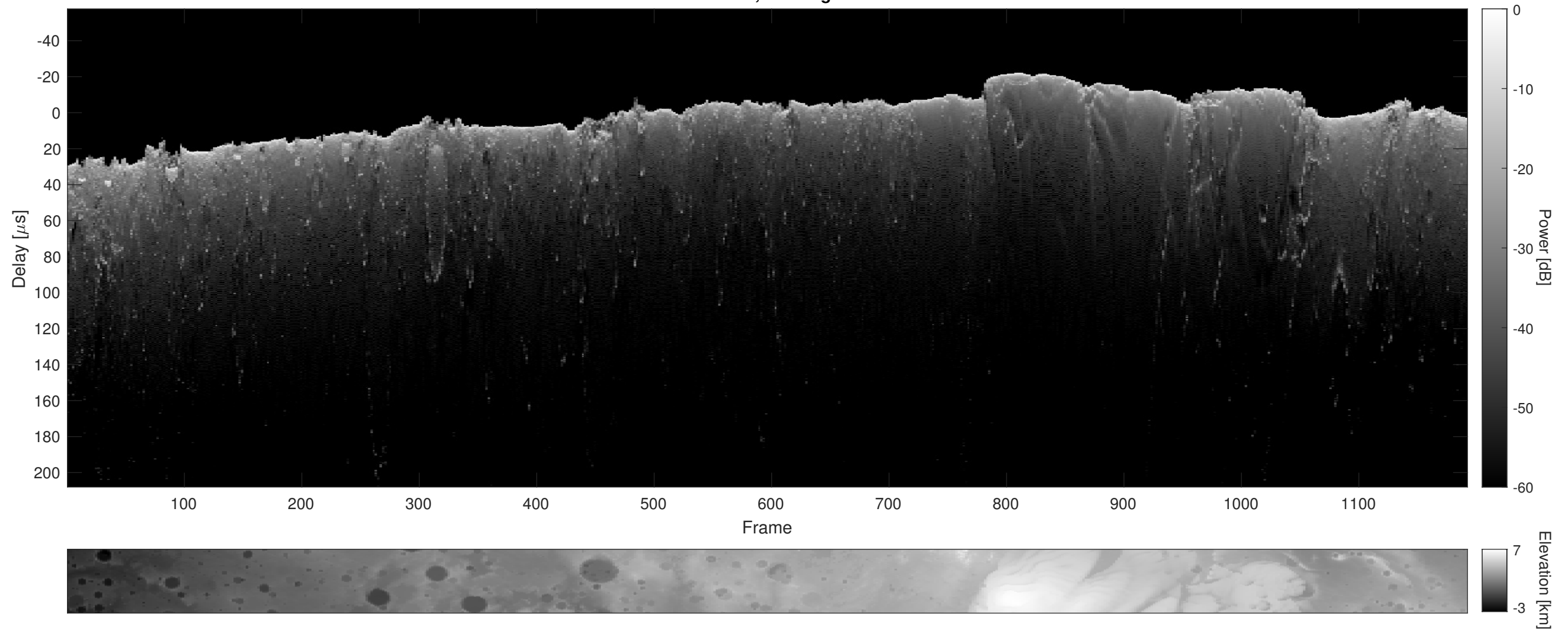
Orbit 8865, Cluttergram
