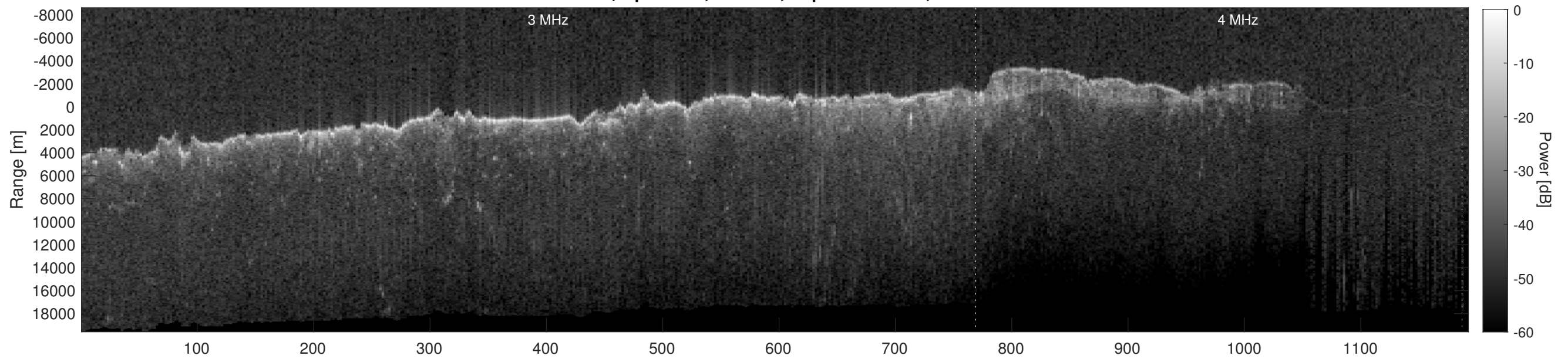
Orbit 8865, Depth-Corrected Cluttergram
