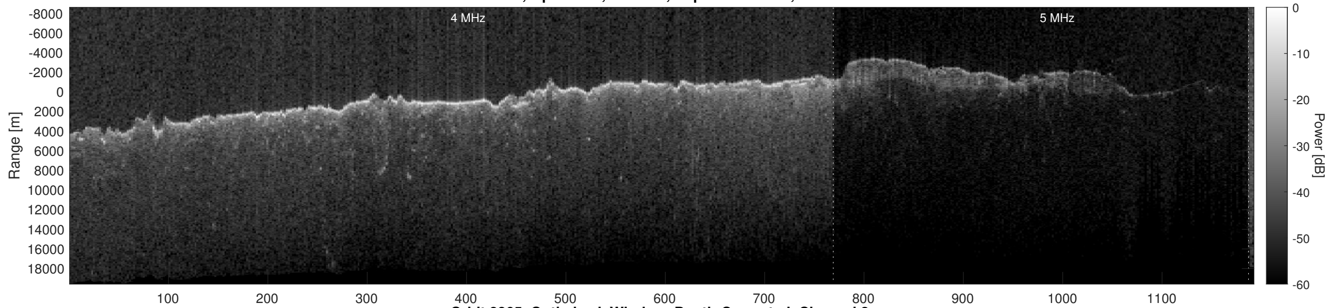
Orbit 8865, Optimized, Window, Depth-Corrected, Channel 2
