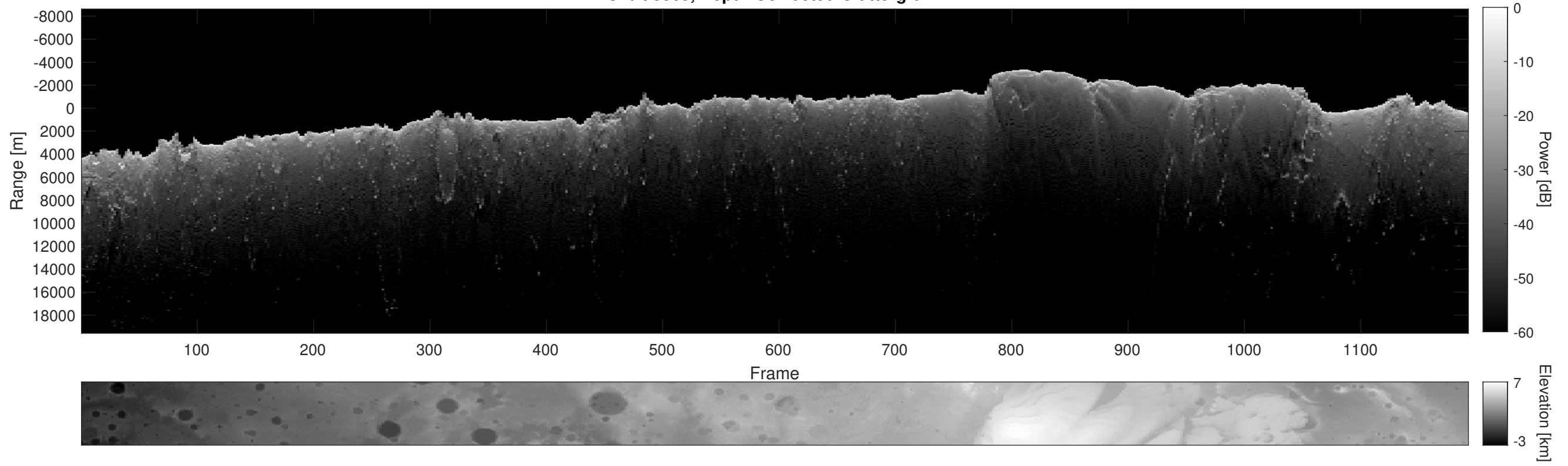
Orbit 8865, Depth-Corrected Cluttergram
