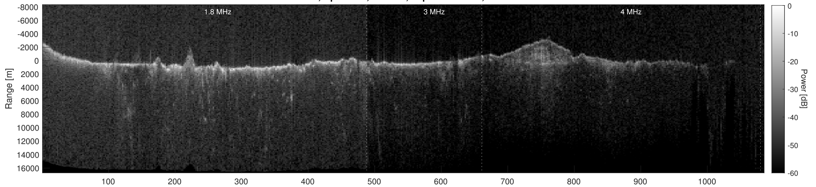
Orbit 8866, Depth-Corrected Cluttergram
