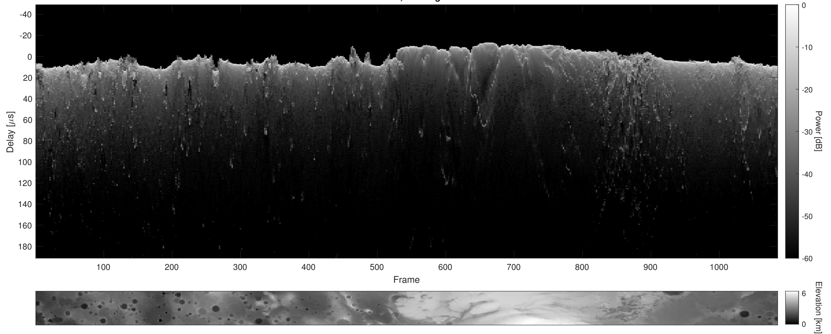
Orbit 8867, Cluttergram
