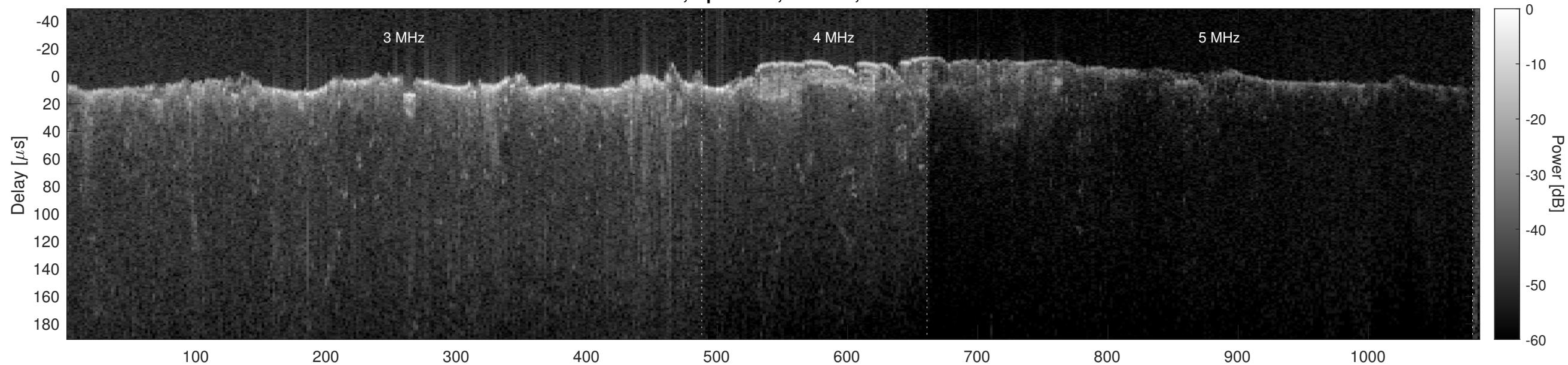
Orbit 8867, Optimized, Window, Channel 2
