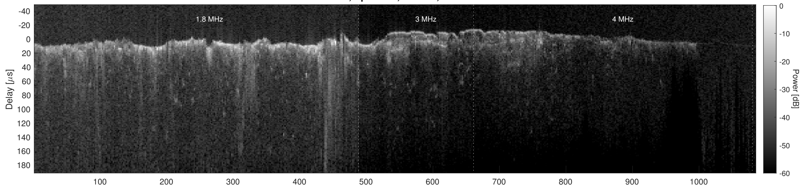
Orbit 8867, Cluttergram
