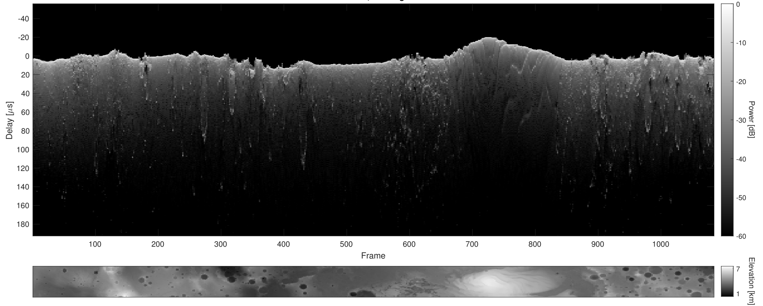
Orbit 8869, Cluttergram
