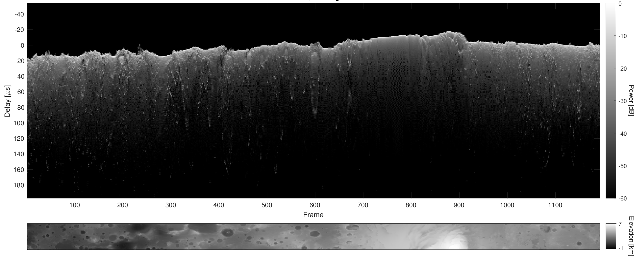
Orbit 8870, Cluttergram
