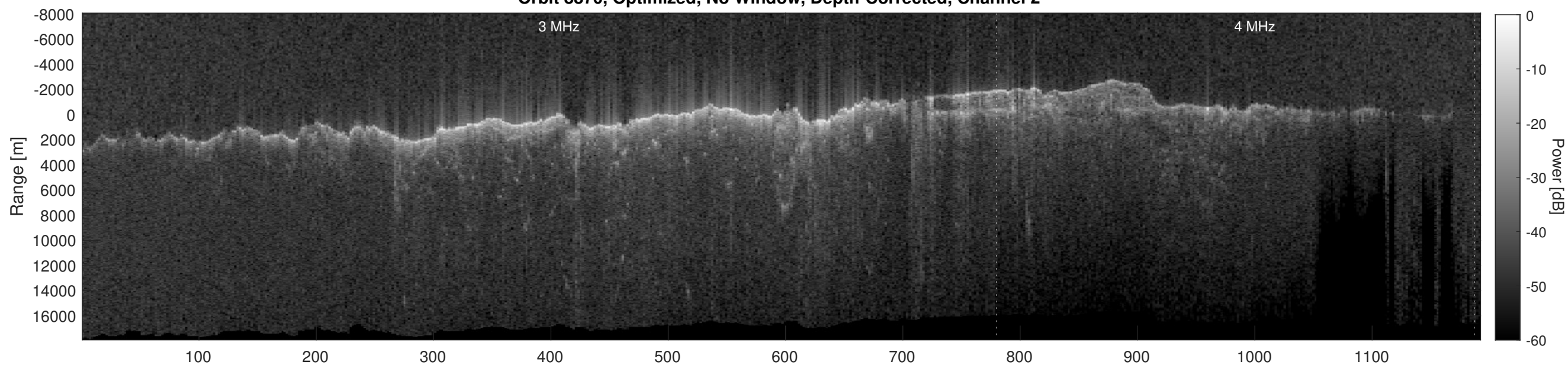
Orbit 8870, Depth-Corrected Cluttergram
