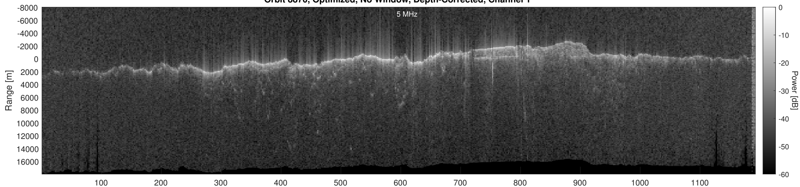
Orbit 8870, Optimized, No Window, Depth-Corrected, Channel 2
