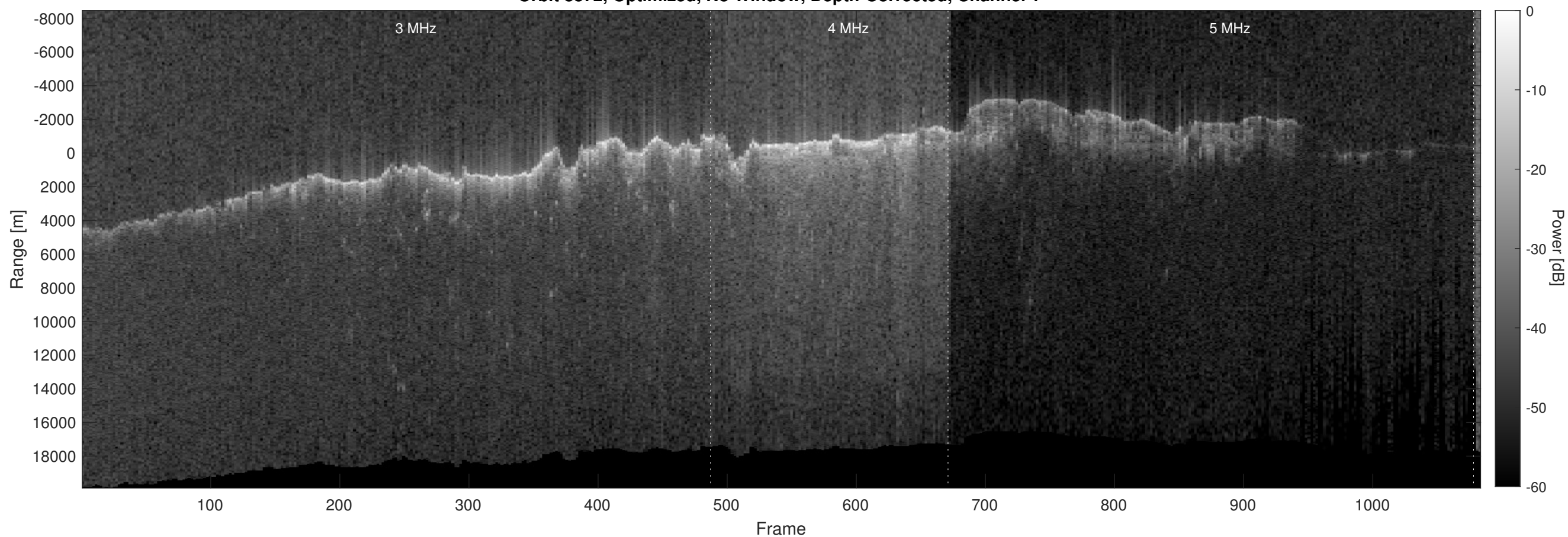
Orbit 8872, Optimized, No Window, Depth-Corrected, Channel 2
