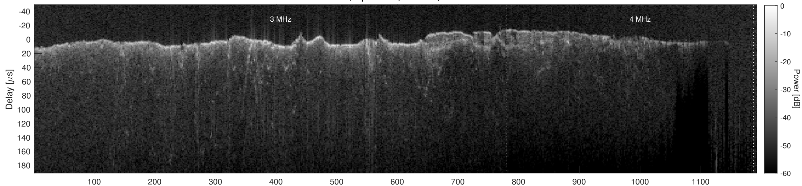
Orbit 8874, Cluttergram
