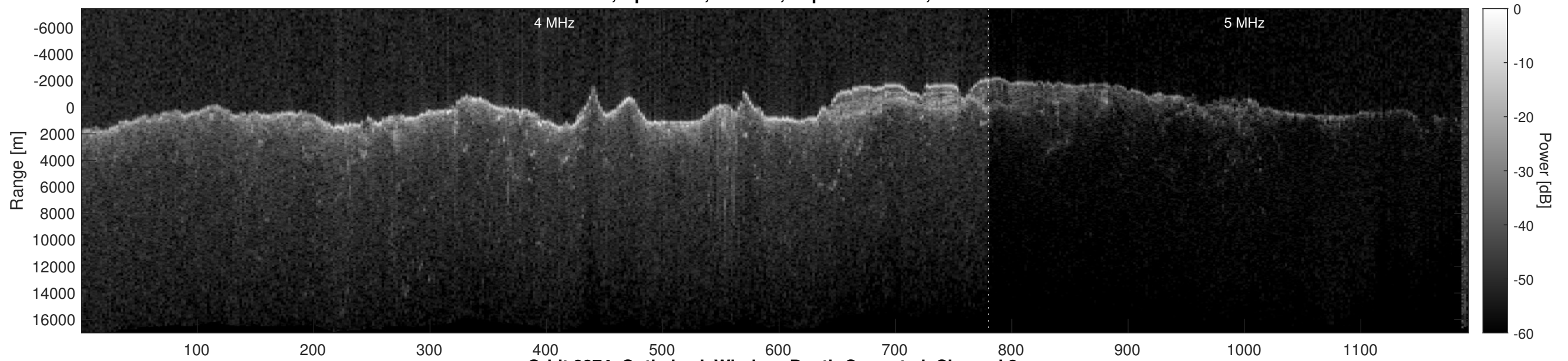
Orbit 8874, Optimized, Window, Depth-Corrected, Channel 2
