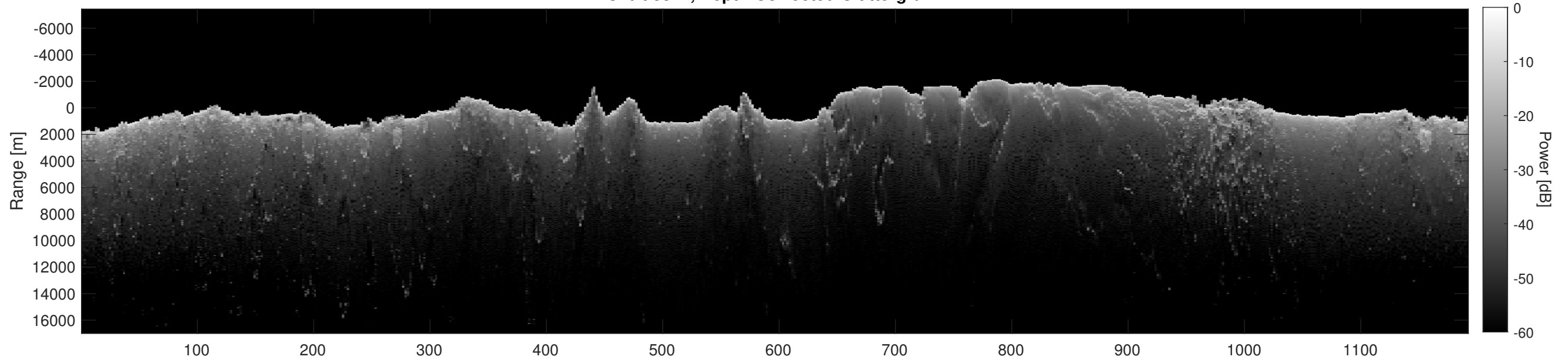
Orbit 8874, Depth-Corrected Cluttergram
