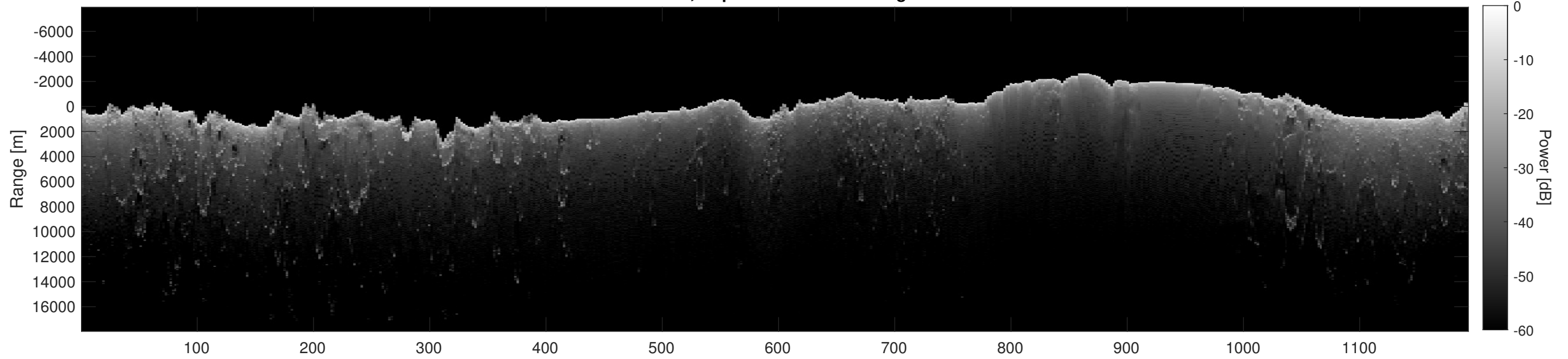
Orbit 8875, Depth-Corrected Cluttergram
