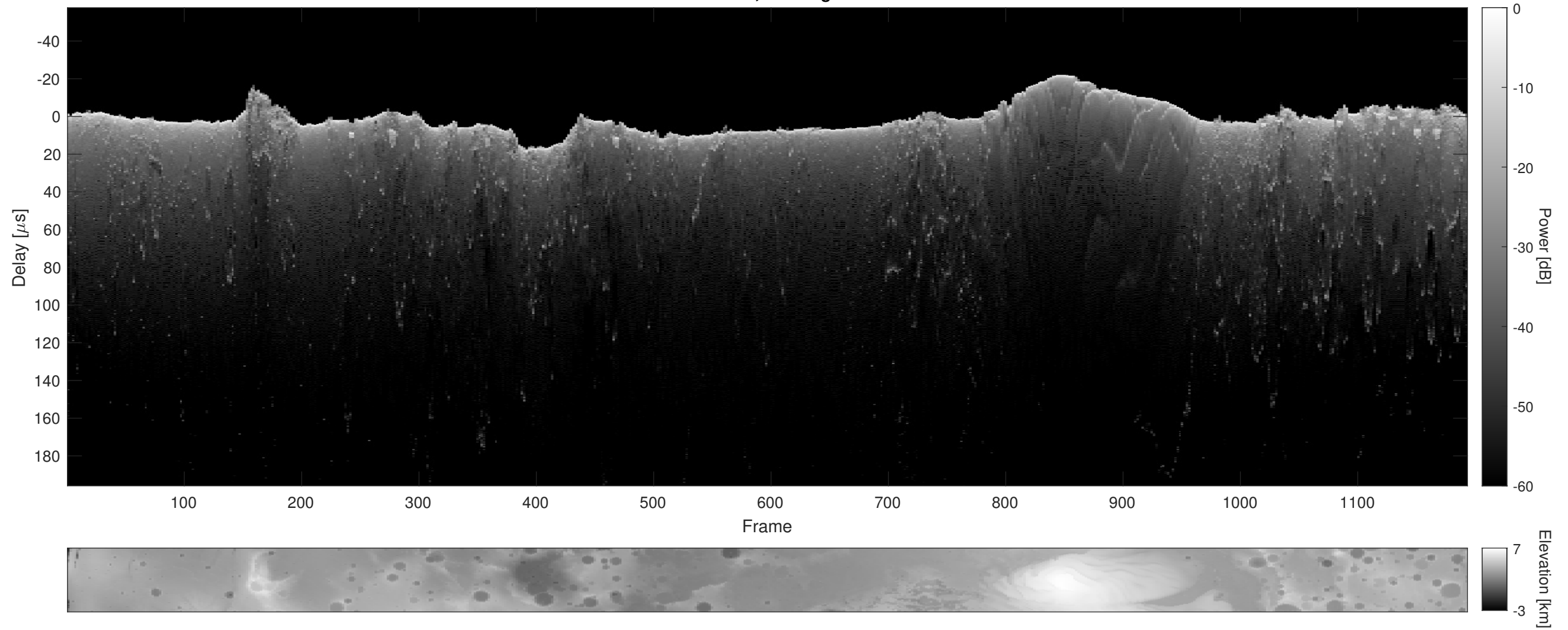
Orbit 8876, Cluttergram
