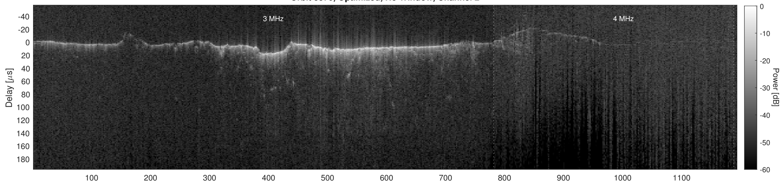
Orbit 8876, Cluttergram
