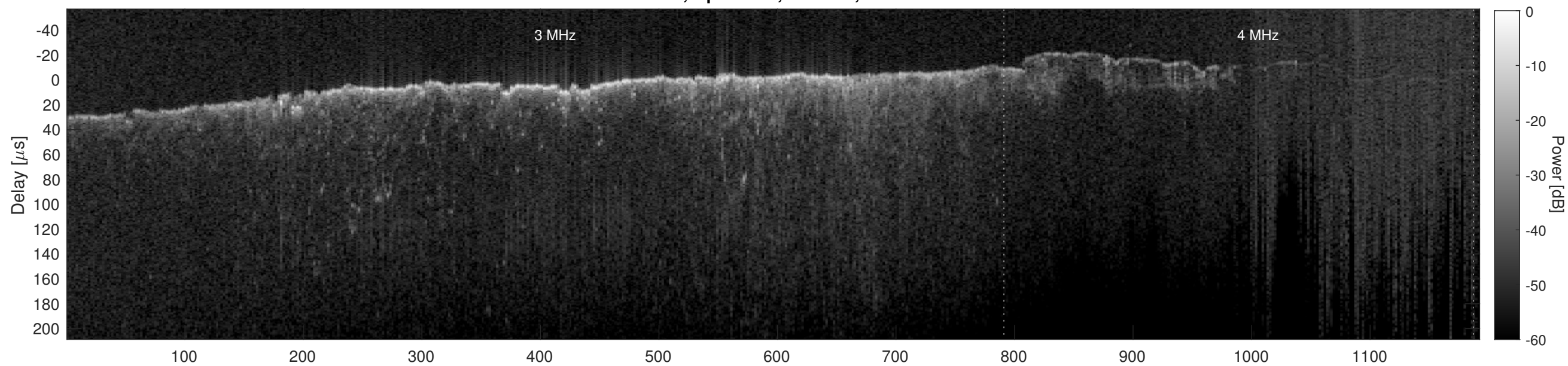
Orbit 8879, Cluttergram
