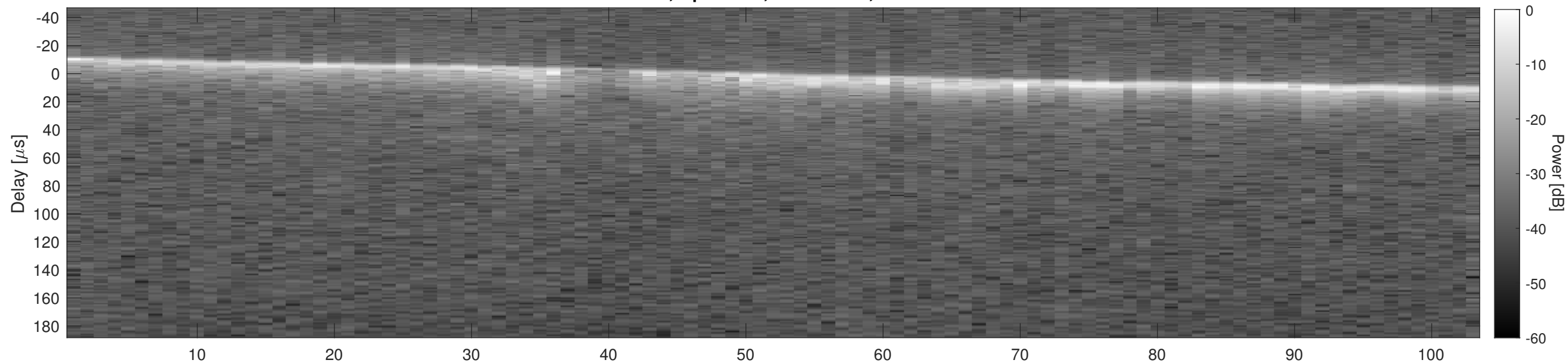
Orbit 8880, Cluttergram
