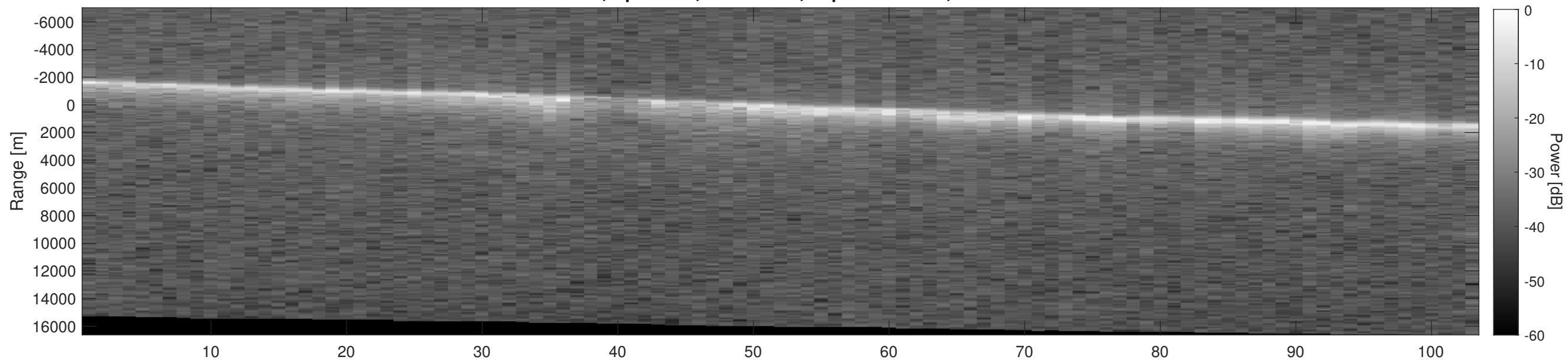
Orbit 8880, Depth-Corrected Cluttergram
