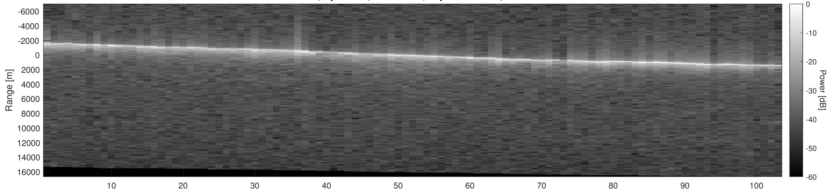
Orbit 8880, Optimized, No Window, Depth-Corrected, Channel 2
