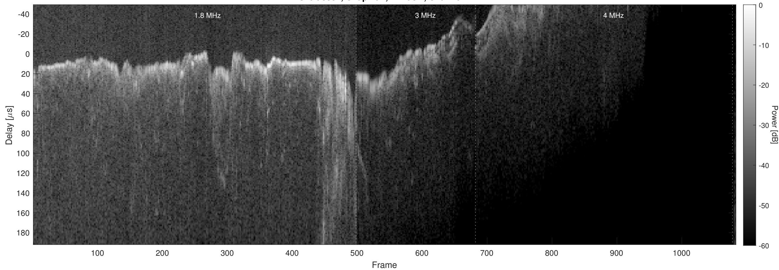
Orbit 8881, Chapman, Window, Channel 2
