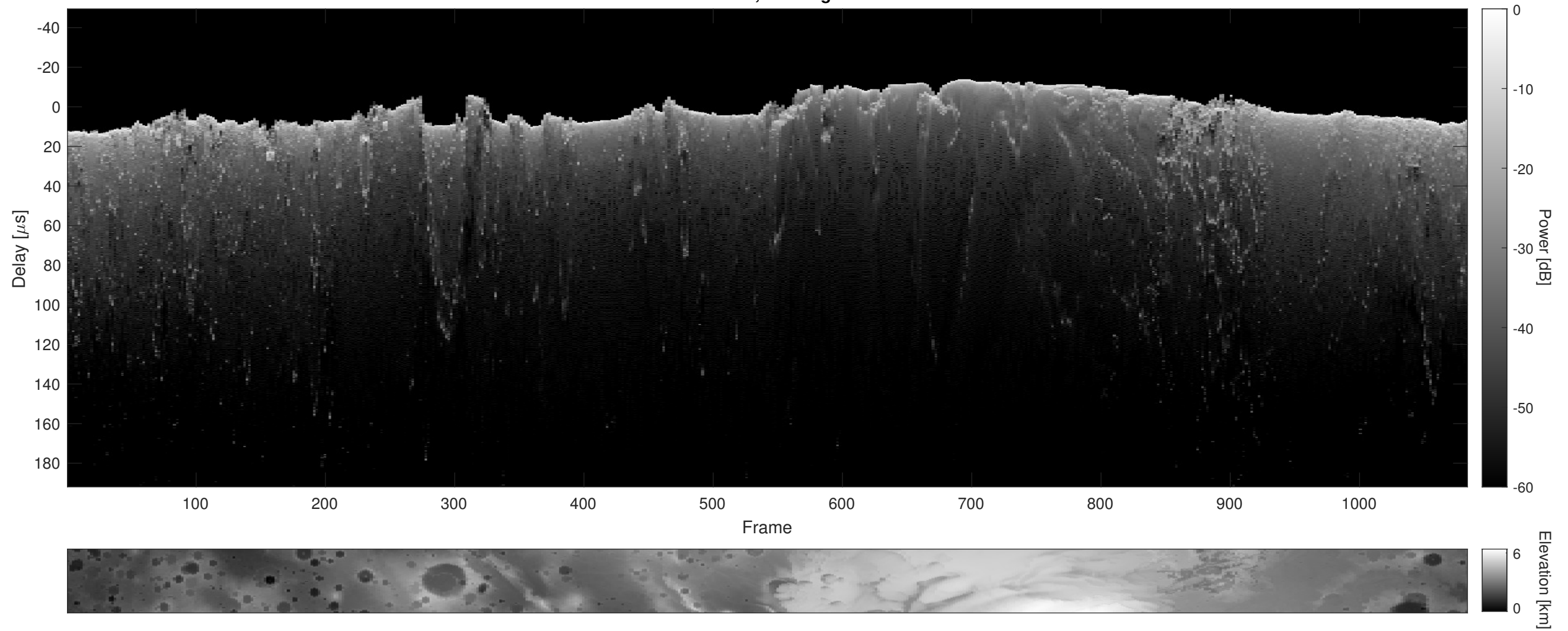
Orbit 8881, Cluttergram
