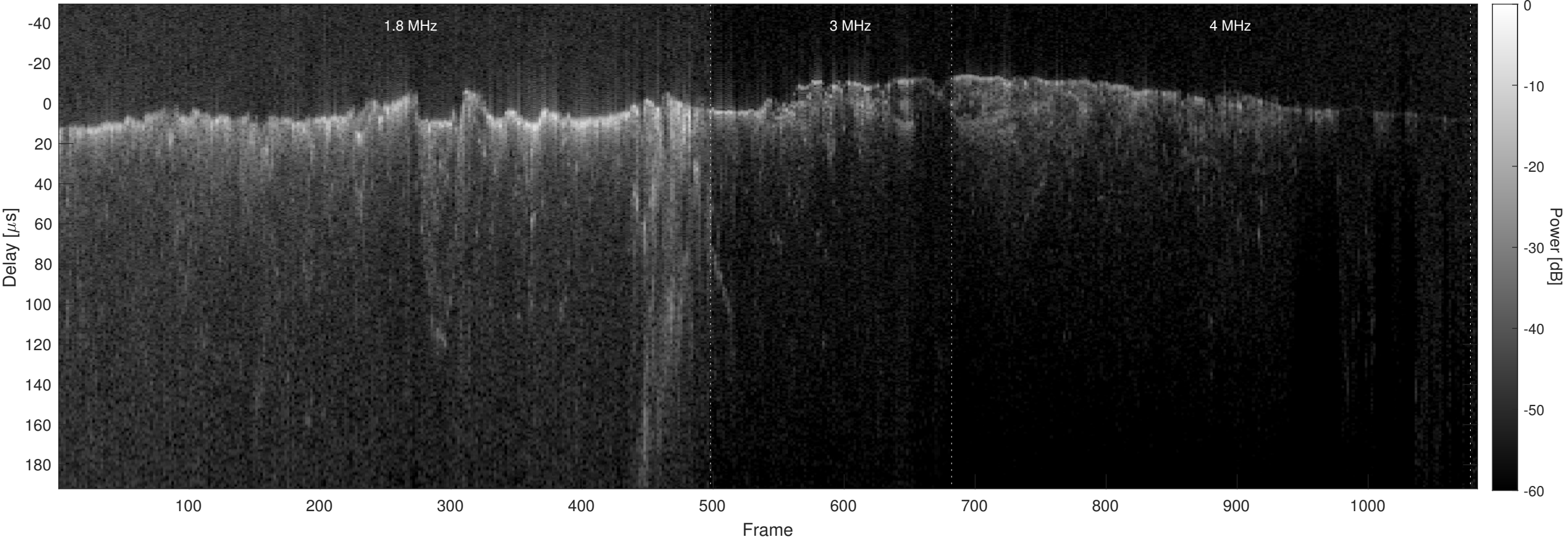
Orbit 8881, Optimized, No Window, Channel 2
