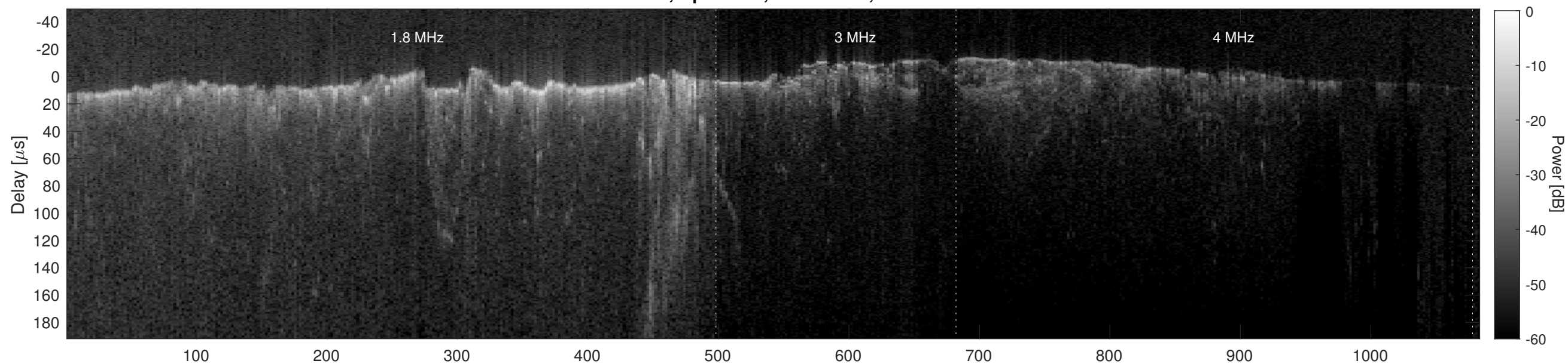
Orbit 8881, Cluttergram
