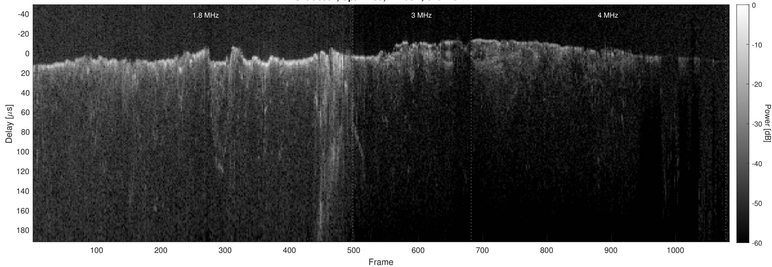
Orbit 8881, Optimized, Window, Channel 2
