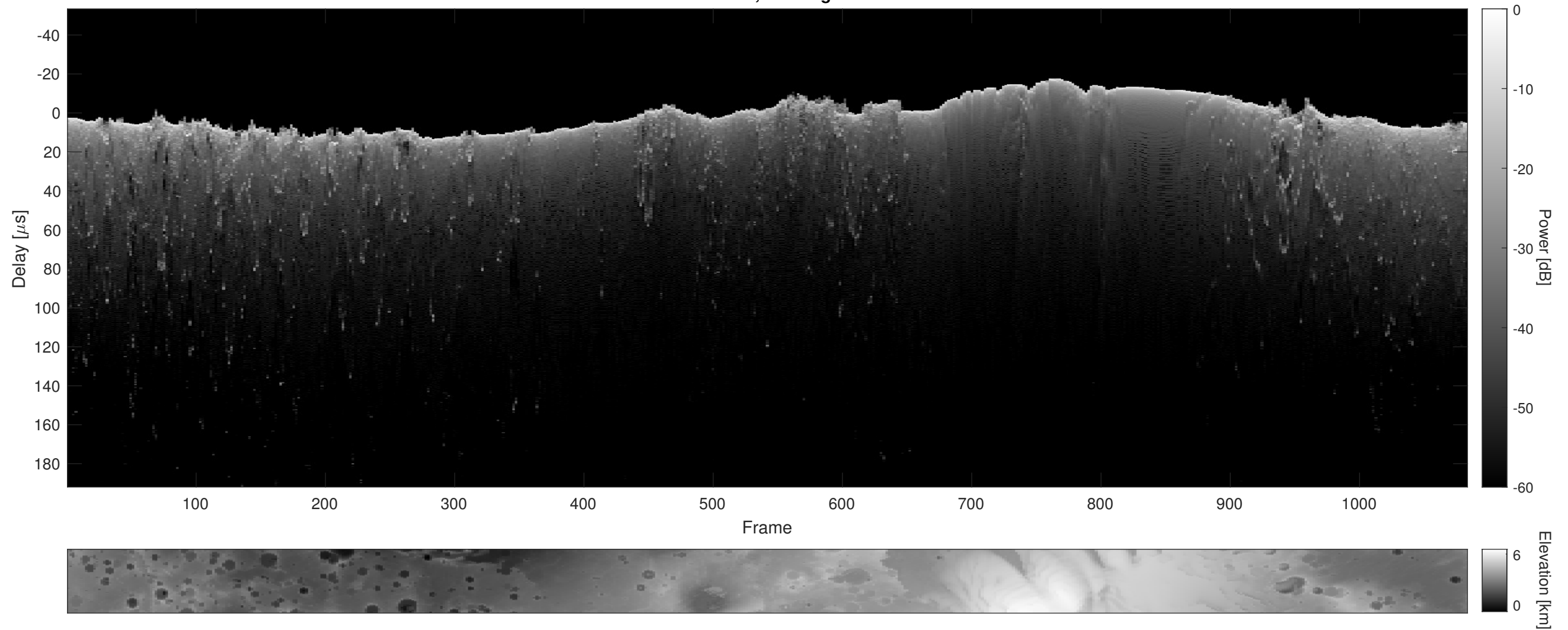
Orbit 8882, Cluttergram
