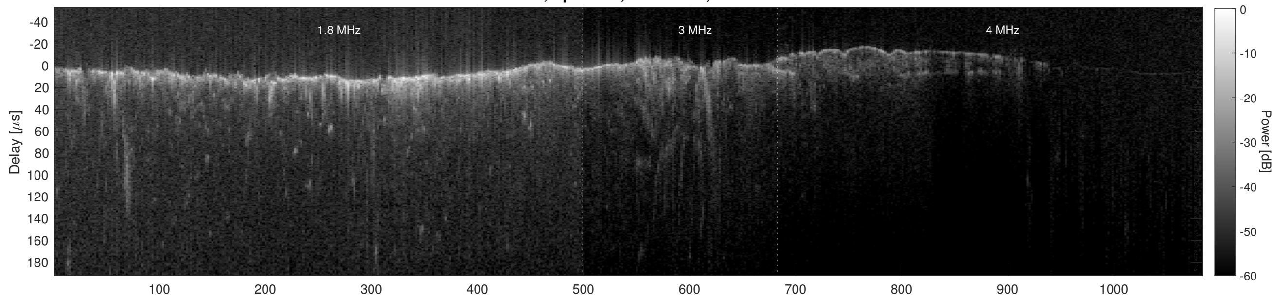
Orbit 8882, Cluttergram
