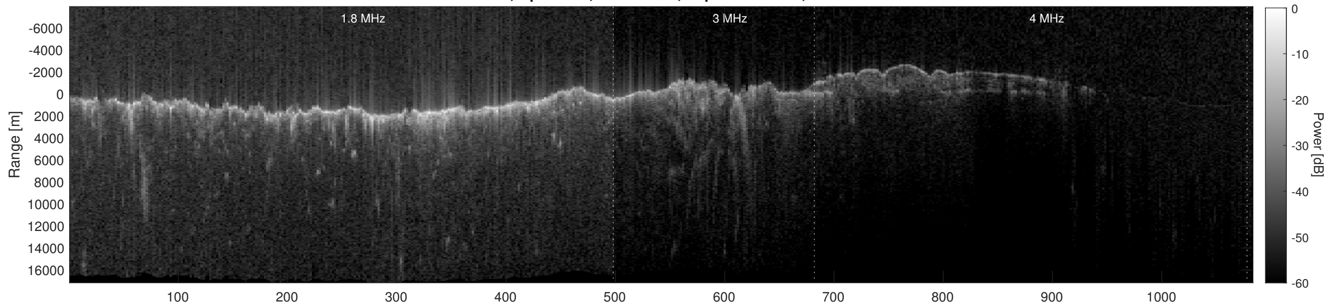
Orbit 8882, Depth-Corrected Cluttergram
