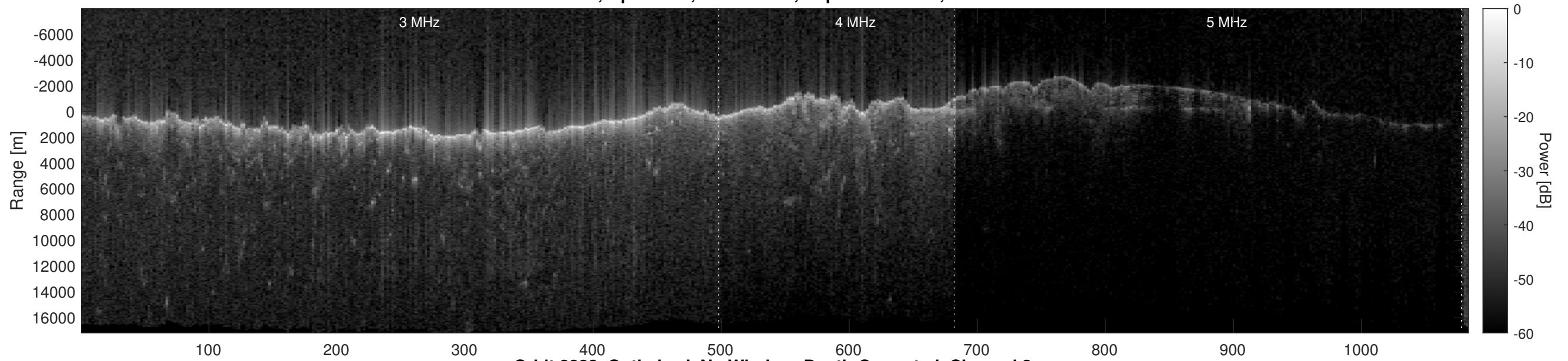
Orbit 8882, Optimized, No Window, Depth-Corrected, Channel 2
