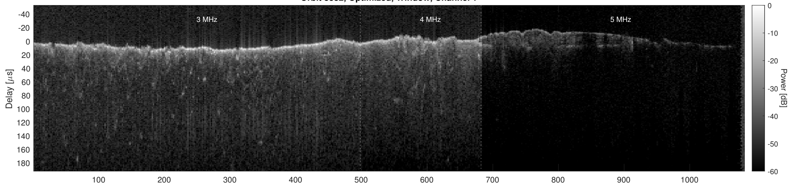
Orbit 8882, Optimized, Window, Channel 2
