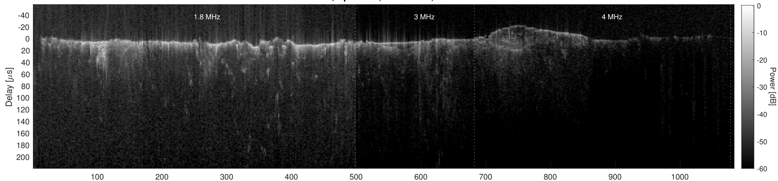
Orbit 8883, Cluttergram
