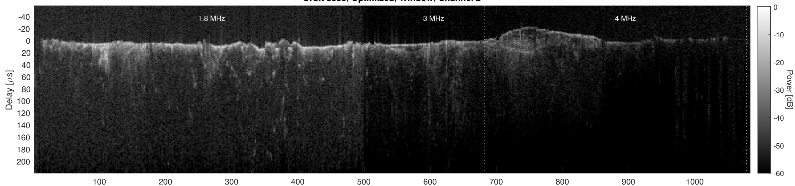
Orbit 8883, Cluttergram
