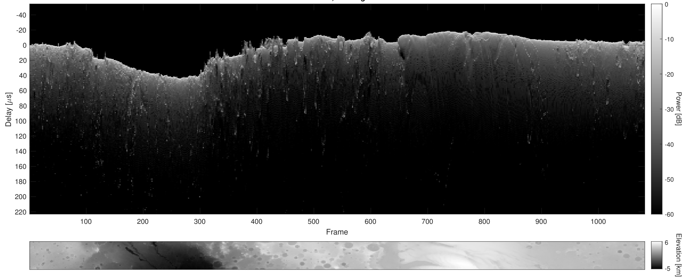
Orbit 8885, Cluttergram
