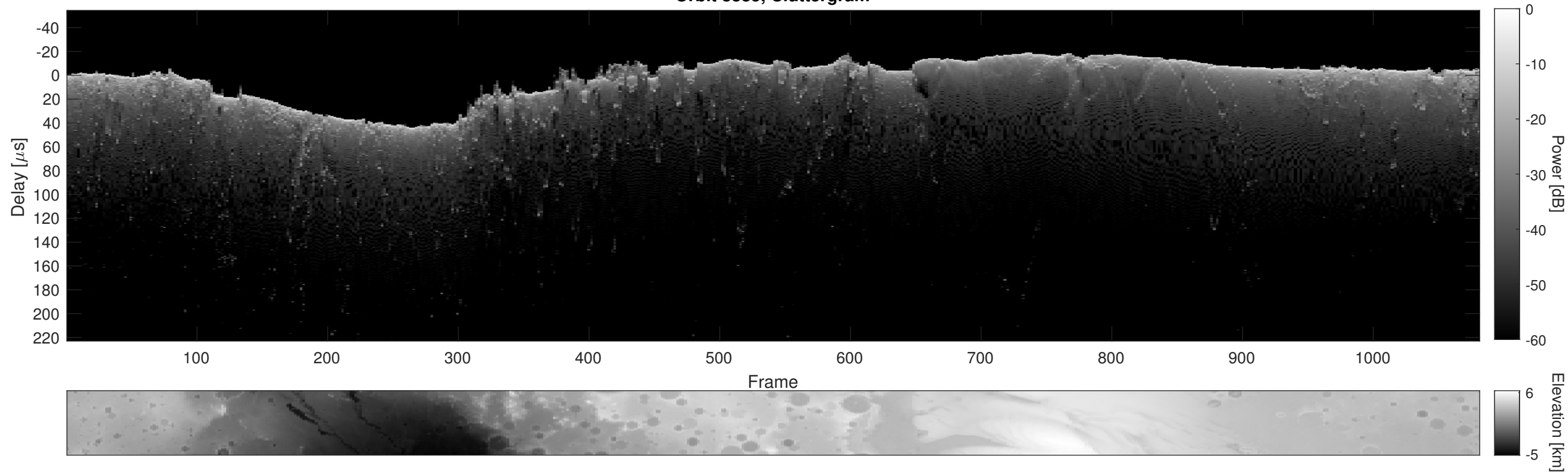
Orbit 8885, Cluttergram
