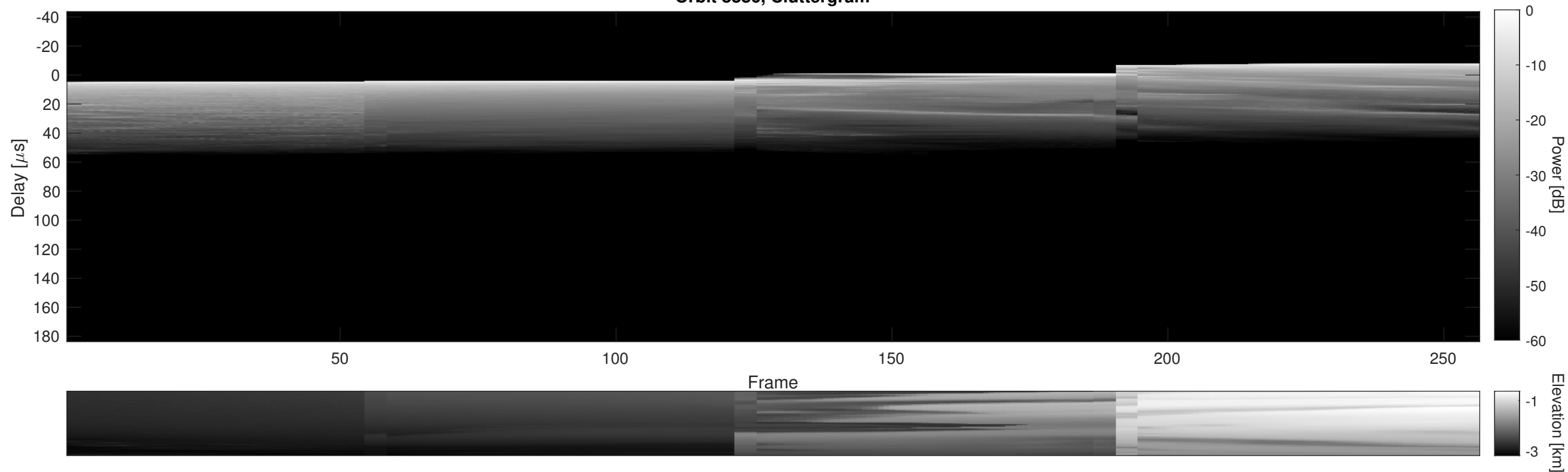
Orbit 8886, Cluttergram
