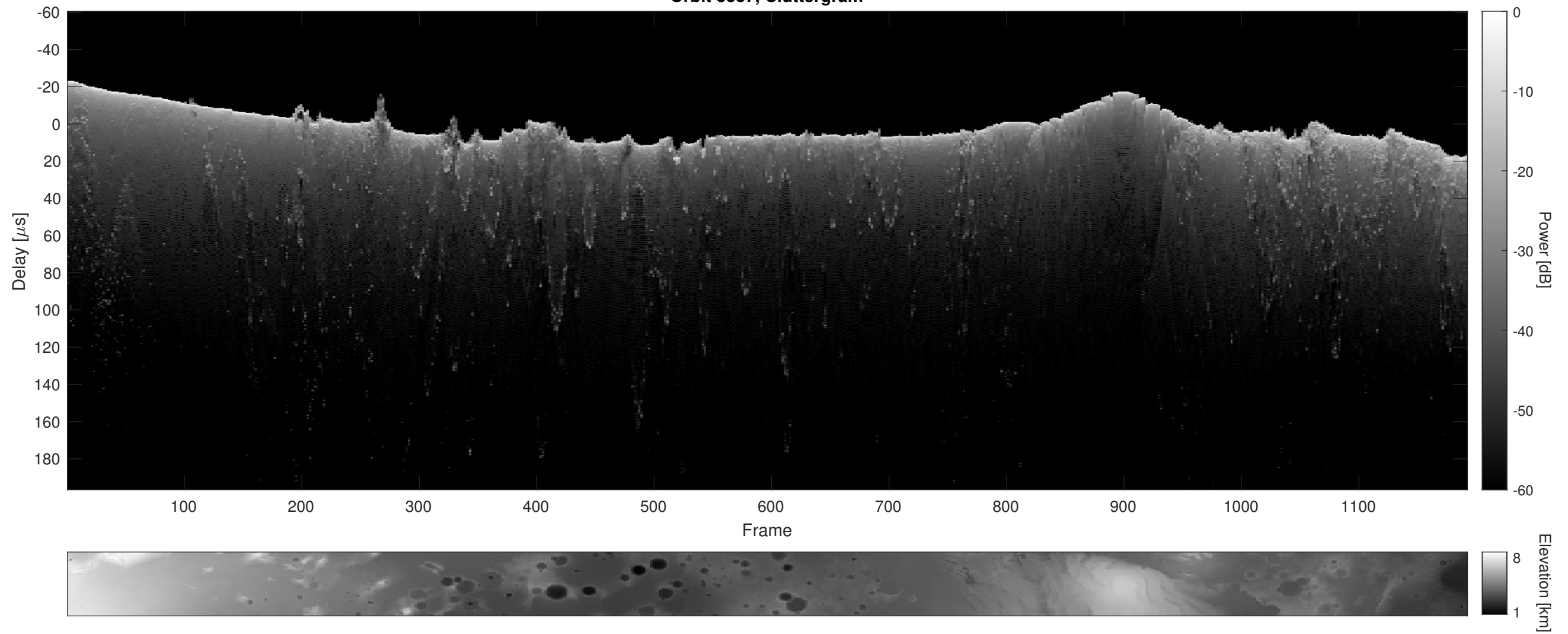
Orbit 8887, Cluttergram
