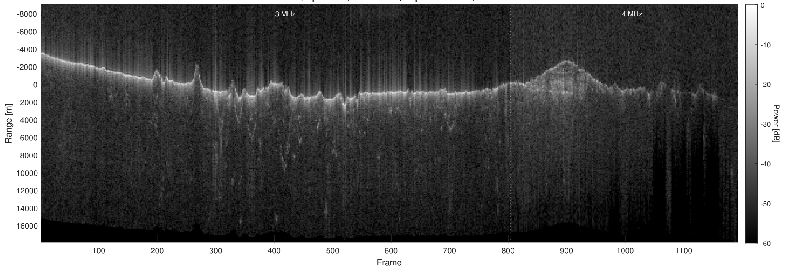
Orbit 8887, Optimized, No Window, Depth-Corrected, Channel 2
